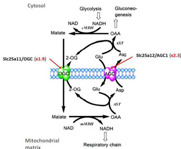
Fig. 3. The malate-aspartate shuttle. AGC1 (Slc25a12, x2.3), the only aspartate/glutamate carrier isoform expressed in synapses, exchanges intra-mitochondrial aspartate (Asp; efflux ) for extra-mitochondrial glutamate (Glu; influx ). In the cytosol, aspartate aminotransferase (AST) converts Asp to oxaloacetic acid (OAA) in a reaction coupled to the conversion of Glu into oxoglutarate (2-OG). The produced OAA is then converted by cytosolic MDH (cMDH) in a NADH-dependent reaction that generates malate and NAD. In this reaction, NADH in the cytosol (inter-membrane space) passes two reducing equivalents to oxaloacetate, producing malate. The generated cytosolic malate generated is then transported into the mitochondrial matrix by OGC (Slc25a11, x1.9) in exchange for intra-mitochondrial 2-OG which arises from mitochondrial MDH (mMDH)-mediated conversion of incoming malate into OAA, passing two reducing equivalents to NAD + and generating NADH in the process, followed by AST-mediated dual conversion of OAA into Asp and intra-mitochondrial Glu into 2-OG. In this process imported cytoplasmic malate passes two reducing equivalents to NAD + and the resulting mitochondrial NADH can then pass electrons directly to the ETC complex I in the inner membrane. The AST-mediated dual conversions reduce the availability of cytosolic Glu while increasing the cytosolic levels of 2-OG and the other side, increase the intra-mitochondrial levels of both Asp and 2-OG, act as feedback loops regulating the activity balance between AGC and OGC which govern the shuttle's dynamics. Here, the electrogenic AGC1 transporter provides directionality so that reducing equivalents are transferred into the mitochondrial matrix (modified from [161]).
